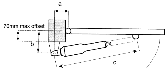
Fig A In swinging gates geometry
